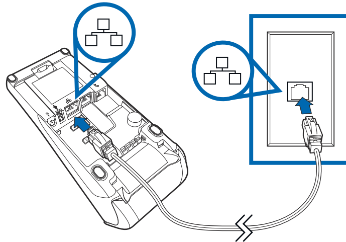
Figure 5 Ethernet Connection
