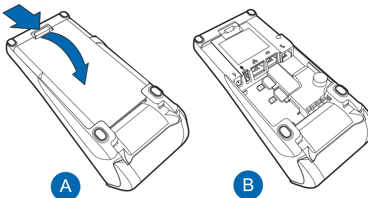
Figure 9 Opening the V200c and V400c Rear Cover
