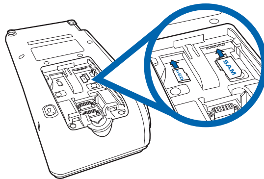
Figure 3 MSAM/uSD Slots
