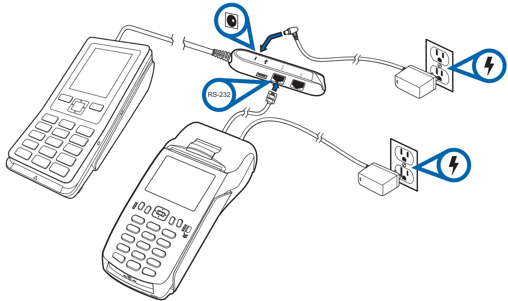
Figure 7 Powering PINpad with External Power Supply
