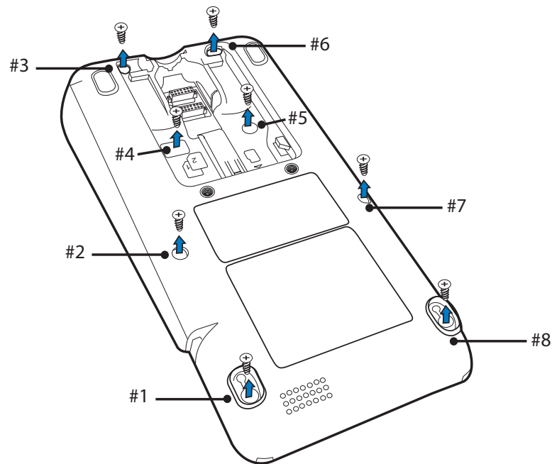
Figure 19 P200 Bottom
