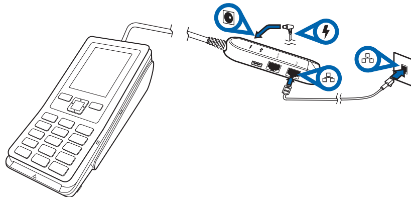
Figure 13 Available Connections on the External Power Brick
