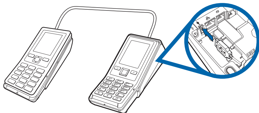
Figure 8 Connecting to V200c Via USB
