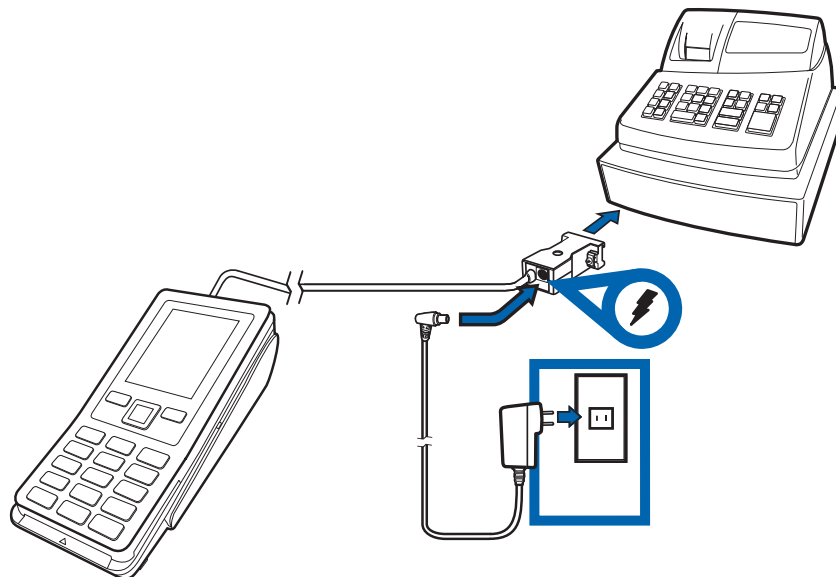
Figure 10 Connecting to RS232-Based Host
