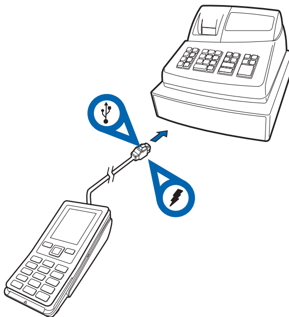
Figure 12 Connecting to USB-Based Host via Powered USB.
