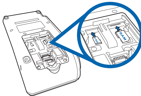
Figure 3 MSAM/uSD Slots
